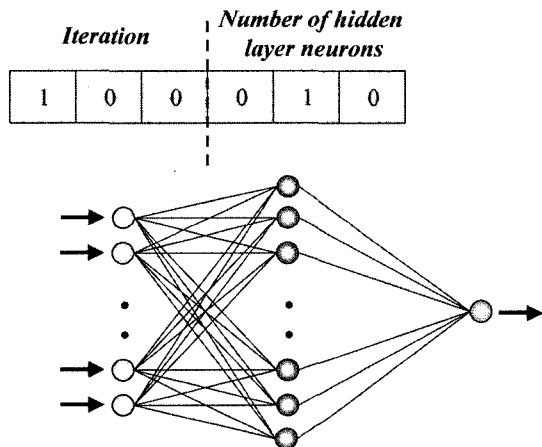
Fig. 1 Binary coding of neural network structure
