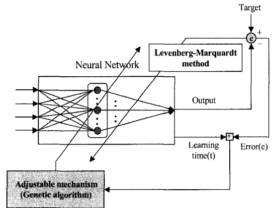
Fig. 2 Structure of optimization using genetic algorithm
