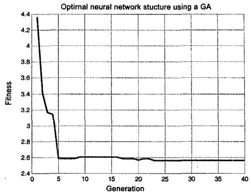
Fig. 4 Search for a optimal neural network structure
