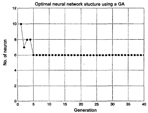
Fig. 5 Optimal number of a neurons in hidden layer
