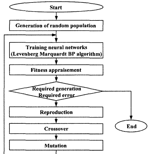
Fig. 3 Operation structure of genetic algorithm
