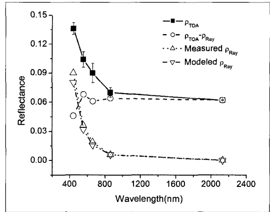
Fig. 2. Observed and modelled reflectance from HYPERION over water pixel.
