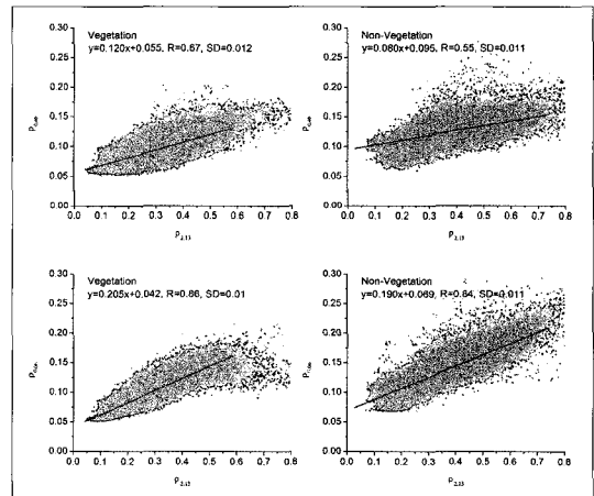
Fig. 3. Visible/SWIR ratio for vegetation (NDVI>0.25) and non-vegetation pixels (NDVI<0.25) at 0.46 and 0.66micron, respectively. Note that reflectance at each wavelength has been corrected Rayleigh scattering and total transmission.
