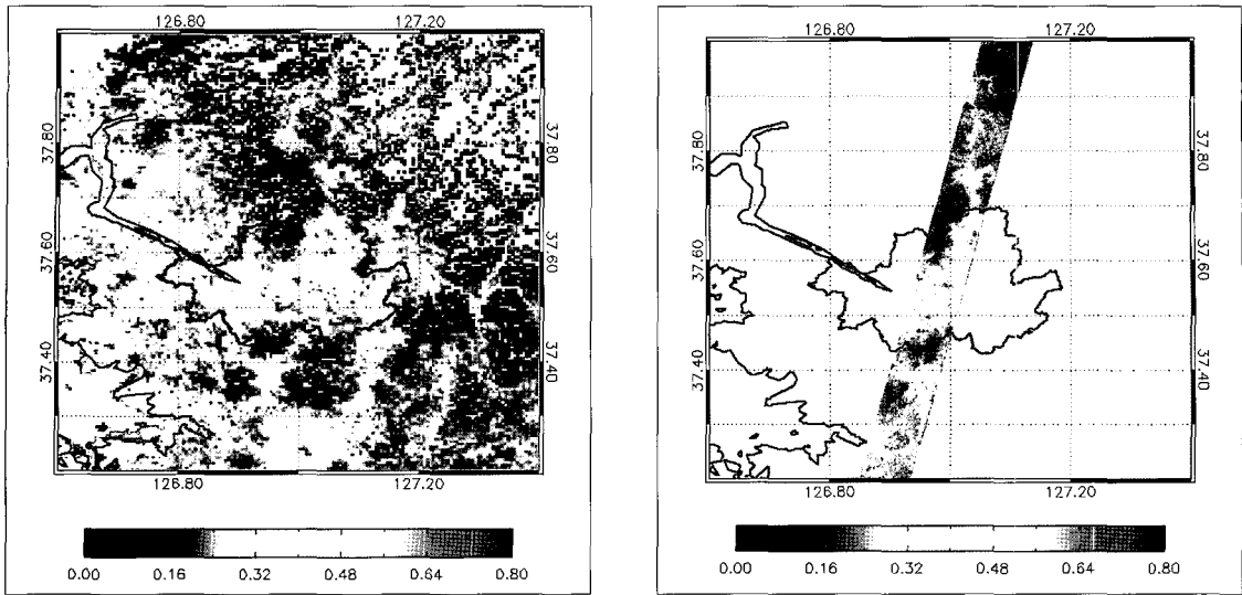
Fig. 4. MODIS retrieved AOT (500m resolution) and HYPERION AOT (30m resolution), respectively.
