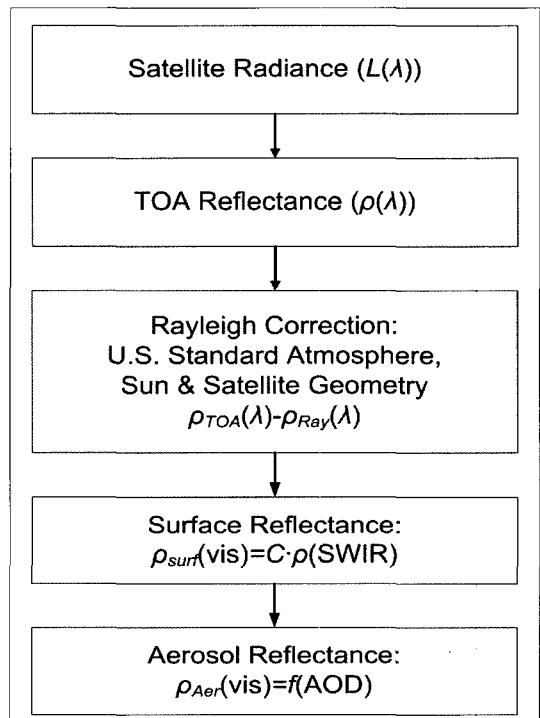
Fig. 1. Flow chart of aerosol detection algorithm.
