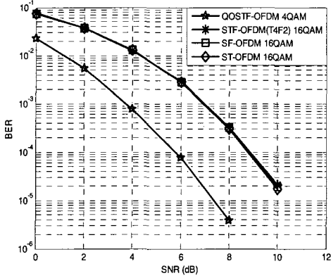
그림 7. Quasi-static Rayleigh fading channels상의 2bits/s/Hz 를 가진 BER성능 비교 Fig. 7. BER performance comparison with 2bits/s/Hz on quasi-static Rayleigh fading channels
