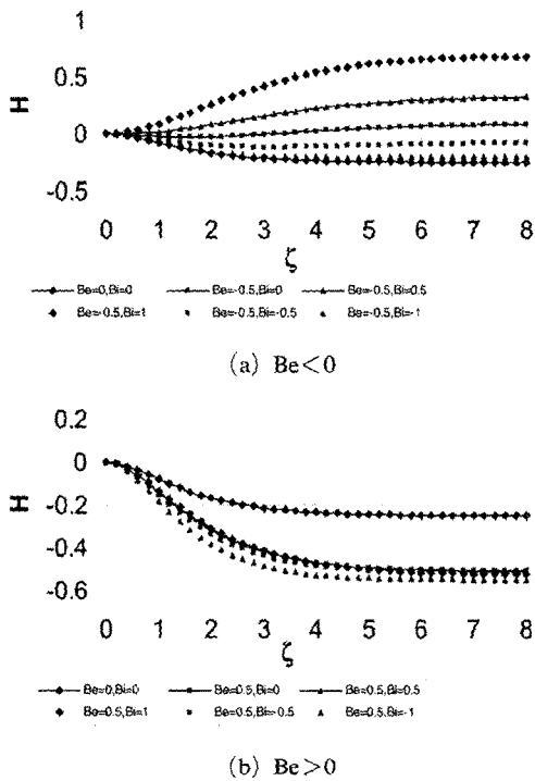
Fig. 3 Steady state profile of the vertical velocity component H for various values of the Hall parameter Be and the ion slip parameter Bi
