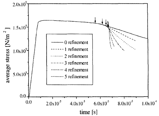
Fig. 4 Average stresses for different meshes. Mark ↓ indicates the inception points of mesh refinements
