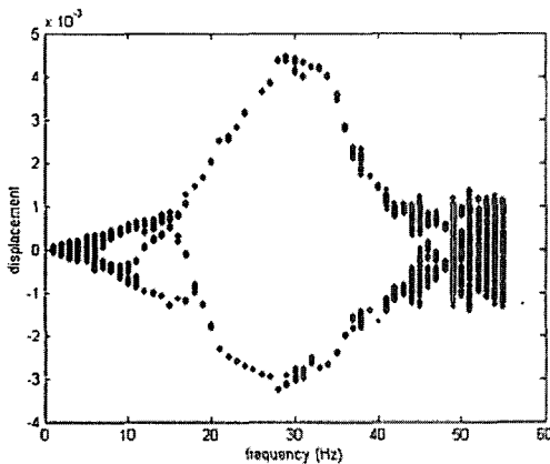
(c) The third mode
