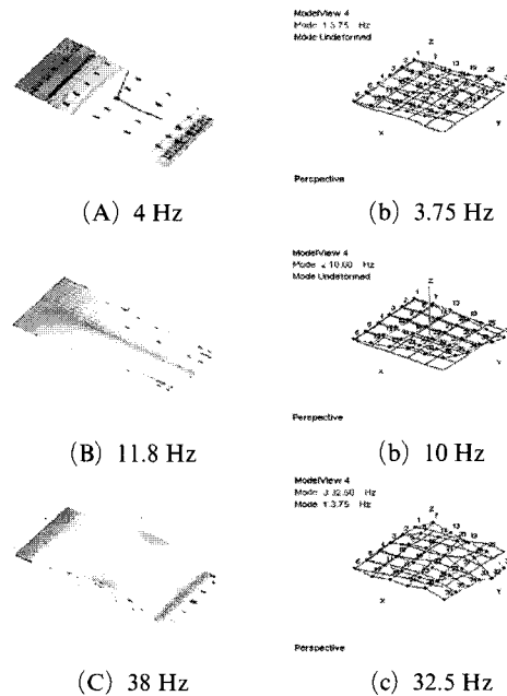
Fig. 3 Vibration modes of the plate; (A), (B) and (C) by Samcef, (a), (b) and (c) by SMS
