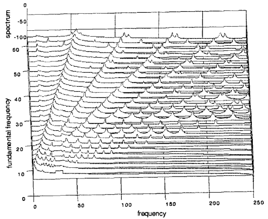
Fig. 9 Waterfall diagram of the plate spectra with linear equation of motion
