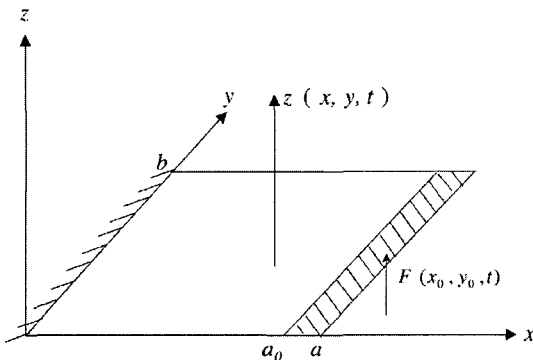
Fig. 1 Schematic of the plate
