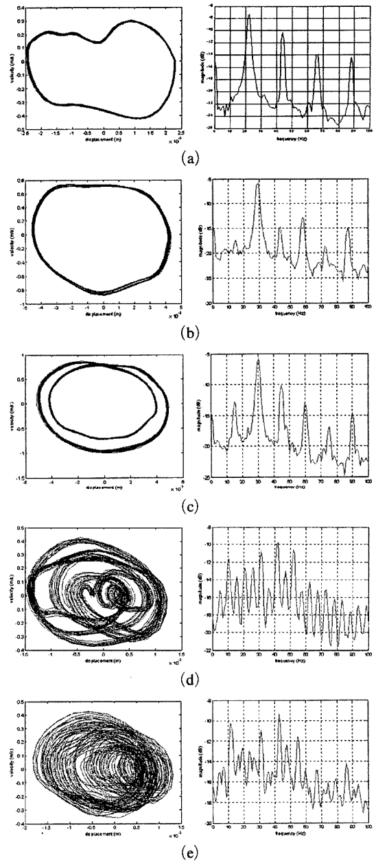
Fig. 7 Phase diagrams and power spectra of the third modal responses for ; (a) 22 Hz, (b) 29 Hz, (c) 30 Hz, (d) 52 Hz and (e) 55 Hz
