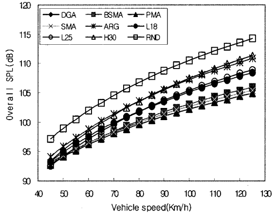
(a) Normal cruising condition
