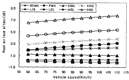
(c) Small truck
