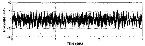
(c) Normal cruising condition at H30 concrete surface road
