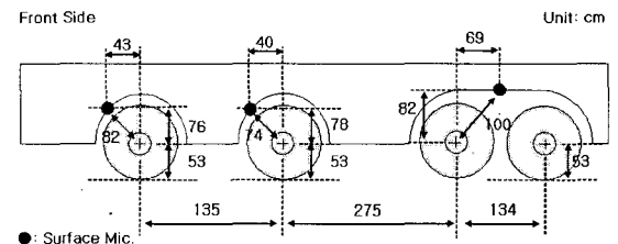
(b) 25ton dump truck
