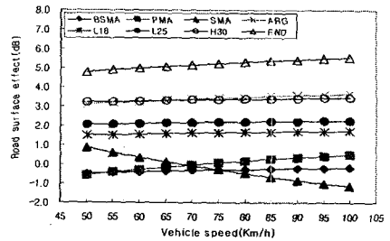
(f) 25ton dump truck (empty condition)
