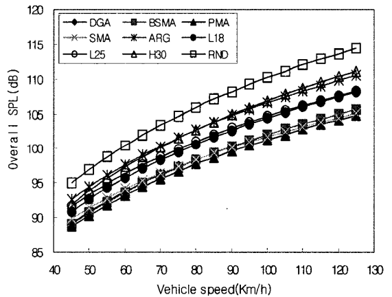
(b) Inertia cruising condition
