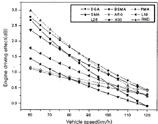
Fig. 6 Difference of noise emission between normal and inertia conditions for large bus
