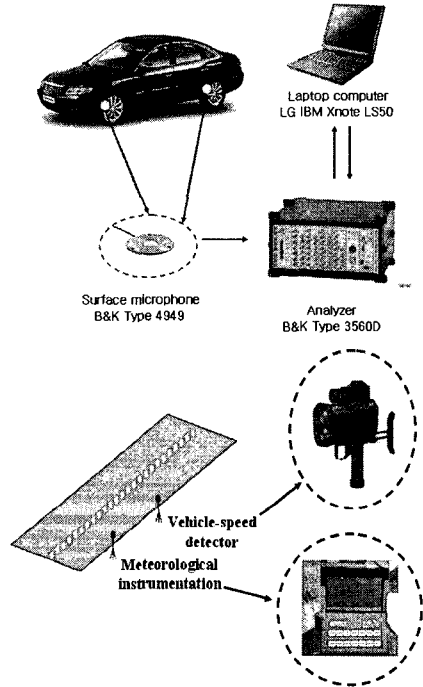
Fig. 2 Configuration of the measurement system
