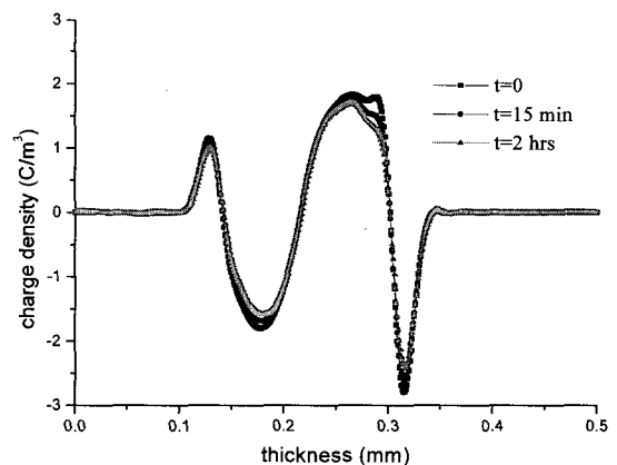
Fig. 2. Charge profiles in ac aged LDPE after the removal of 50 kV/mm dc electric stress.
