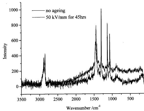
Fig. 5. Raman spectra of ac aged LDPE.
