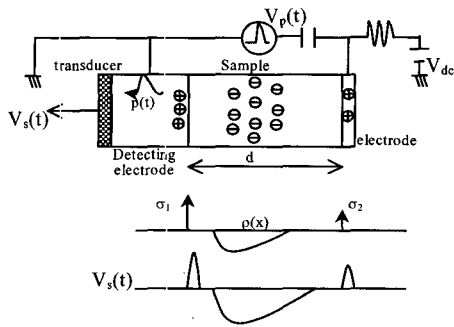
Fig. 1. Schematic diagram of PEA.
