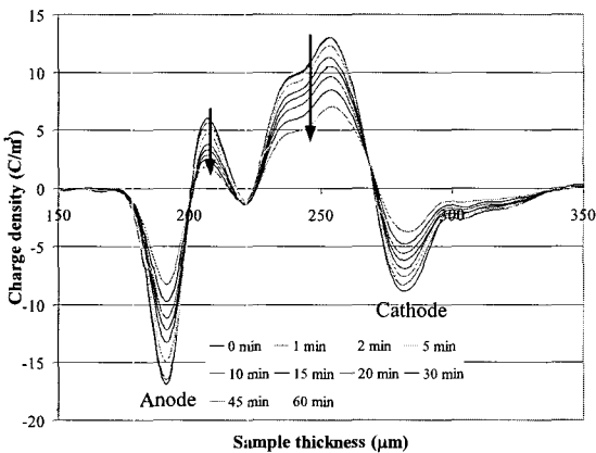
Fig. 8. Charge decay dynamics in 100 kGy irradiated sample after the removal of the applied voltage.
