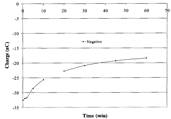
Fig. 11. Charge decay in 100 kGy irradiated sample after being stressed at 50 kV/mm for 60 minutes.
