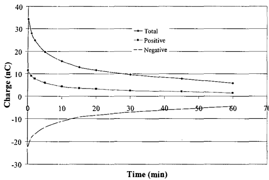
Fig. 7. Charge decay in control sample after being stressed at 50 kV/mm for 60 minutes.
