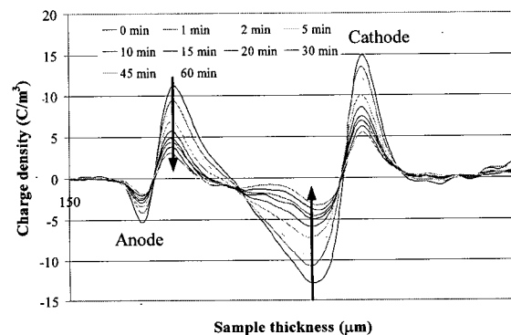
Fig. 6. Charge decay dynamics in control sample after the removal of the applied voltage.
