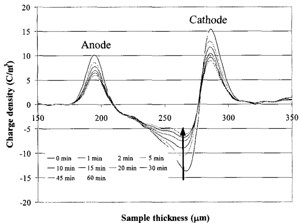
Fig. 10. Charge decay dynamics in 100 kGy irradiated sample in nitrogen gas.
