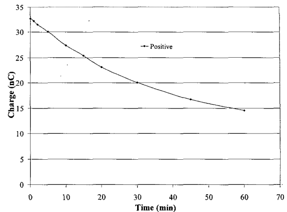
Fig. 9. Charge decay in 100 kGy irradiated sample after being stressed at 50 kV/mm for 60 minutes.
