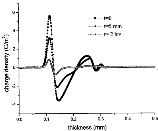
Fig. 3. Charge profiles in unaged LDPE after the removal of 50 kV/mm dc electric stress.
