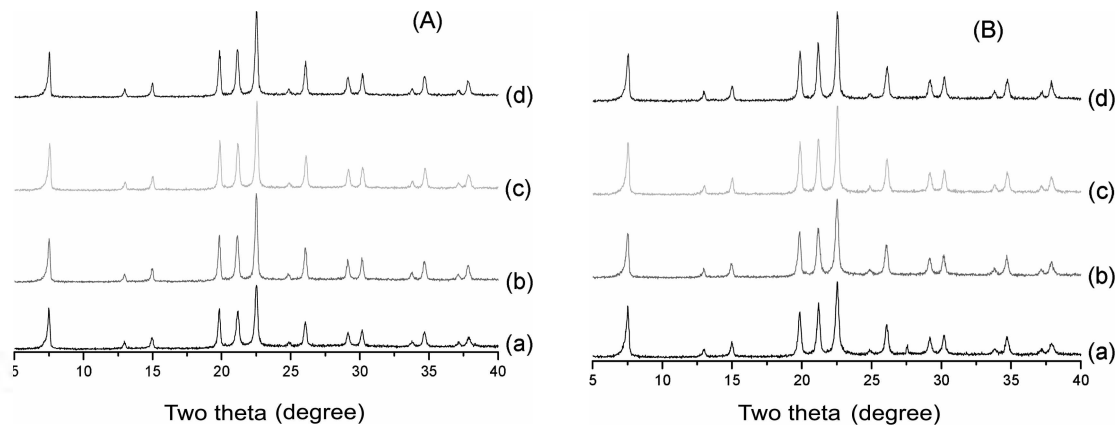
Fig. 1. XRD patterns of FAPO-5 molecular sieves synthesized at 170 °C from same reactant gel (Al 2 O 3 :1.05P 2 O 5 :0.04FeO:1.2TEA:50H 2 O, pH=3.6) in various conditions: (A) microwave crystallization for (a) 8 min, (b) 15 min (c) 30 min, and (d) 60 min; (B) conventional electrical crystallization for (a) 3h, (b) 6h (c) 12h, and (d) 24h.
