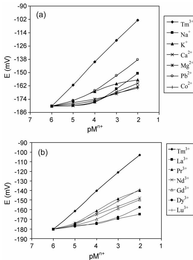
Figure 1. (a, b) Potential responses of the different ion-selective electrodes based on DADS.
