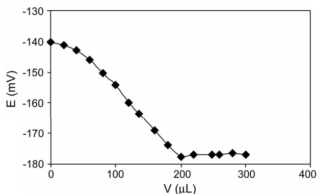
Figure 5. Potentiometric titration curve of 20.0 mL of 1.0 \times 10^{-4} M Tm(III) with 1.0 \times 10^{-2} M of EDTA, using the proposed membrane sensor as an indicator electrode.
