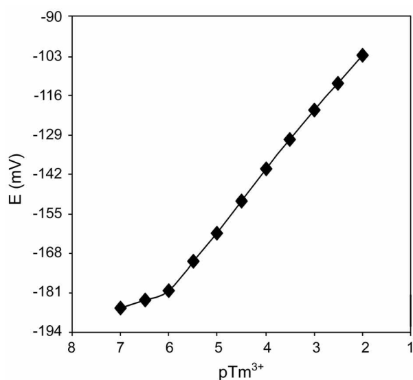
Figure 2. Calibration curve of Tm(III) membrane sensor based on DADS for the membrane no. 6.
