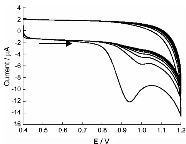
Figure 2. Successive cyclic voltammograms of 5.0 \times 10^{-6} mol/L 6-BAP at SWNT-DCP modified GCE in 0.1 mol/L phosphate buffer ( \text{pH} 7.0 ). Scan rate: 100 mV/s.
