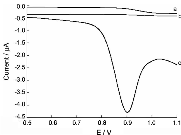
Figure 3. DP voltammograms of 5.0 \times 10^{-7} mol/L 6-BAP in 0.1 mol/L phosphate buffer ( \text{pH} 7.0 ) after 3-min open-circuit accumulation. (a): at unmodified GCE, (b): at DCP film modified GCE, and (c): at SWNT-DCP modified GCE. The DPV parameters: pulse amplitude = 50 mV, scan rate = 20 mV/s, pulse width = 50 ms.
