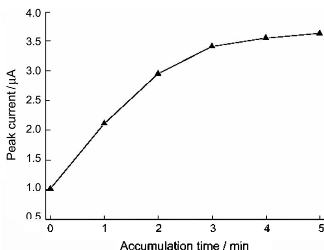
Figure 5. Influence of accumulation time on the oxidation peak current of 5.0 \times 10^{-7} \text{ mol/L} 6-BAP. Other conditions are the same as in Fig. 3c.
