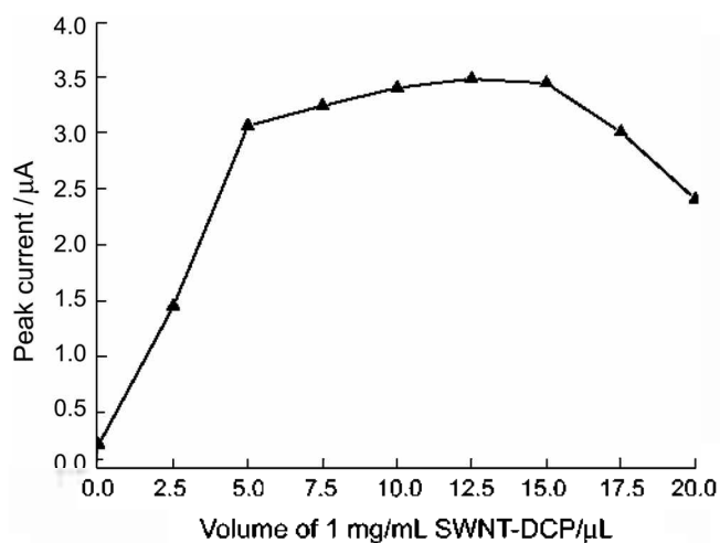
Figure 4. Effect of the volume of the SWNT-DCP suspension on the oxidation peak current of 5.0 \times 10^{-7} \text{ mol/L} 6-BAP. Other conditions are the same as in Fig. 3c.
