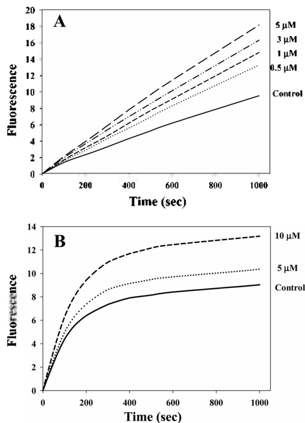
Figure 1. Stimulation of the peptide-hydrolyzing m-calpain activity by \alpha -synuclein. The LLVY-AMC cleaving calpain activity was continuously monitored at either 15 °C (A) or 37 °C (B) by measuring the fluorescence of AMC at 460 nm upon excitation at 380 nm in the presence of various concentrations of \alpha -synuclein as indicated on the panels. The fluorogenic substrate (150 \mu M) was incubated with 20 nM m-calpain in the digestion buffer of 50 mM Tris-Cl, pH 7.5, containing 1 mM EDTA, 0.1 M KCl, 1 mM DTT, and 20 mM CaCl 2 .
