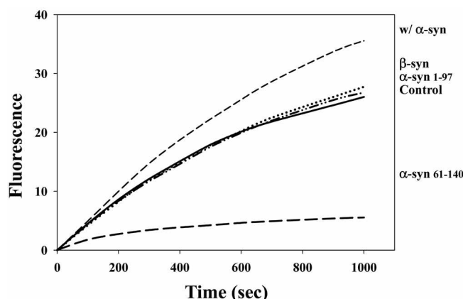
Figure 4. m-Calpain activities in the presence of the modified synucleins. The peptide-hydrolyzing m-calpain activities were monitored with the fluorescence at 460 nm for the reactions of 20 nM m-calpain and 150 mM LLVY-AMC at 25 °C in the presence of 5 \mu M \alpha -synuclein and its related proteins such as \beta -synuclein, \alpha -syn1-97, and \alpha -syn61-140 as indicated on the panel.
