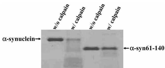
Figure 5. Calpain digestions of \alpha -synuclein and \alpha -syn61-140. \alpha -Synuclein and \alpha -syn61-140 were subjected to m-calpain (0.33 \mu M) digestion in the digestion buffer at 37 ^{\circ} C for 2 hours. Undigested \alpha -synuclein and \alpha -syn61-140 are shown on lanes 1 and 3, respectively, as indicated by arrows. Digestions of \alpha -synuclein and \alpha -syn61-140 by m-calpain were shown on lanes 2 and 4, respectively.
