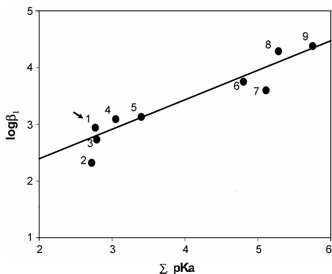
Figure 1. Correlation of the stability constants ( \log \beta_1 ) of the europium(III) complexes and the acid constants ( \Sigma pK_a ) of some bidentate ligands; 1. pipecolinate, 2. L-proline, 3. trans-4-hydroxy-L-proline, 4. croconate, 5. \alpha -piccolinated N-oxide, 6. glutarate, 7. \alpha -piccolinate, 8. malonate, 9. 1,4-cyclohexanedicarboxylate
