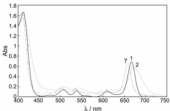
Figure 2. UV-vis spectra of 1 , 2 and 7 in \text{CHCl}_3 .
