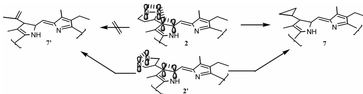
Figure 1. The difference between chlorin 2 and 2' in homoconjugation effect with parent ring and their ring cleavage.
