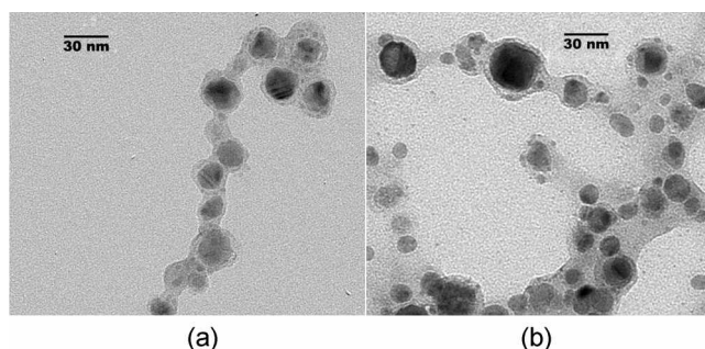
Figure 5. TEM images of Cu nanoparticles after aging 60 days. The conditions of initial irradiation are 50 mJ/pulse (a) and 150 mJ/pulse (b) for 30 min, and that of the second irradiation is 250 mJ/pulse for 50 min.
