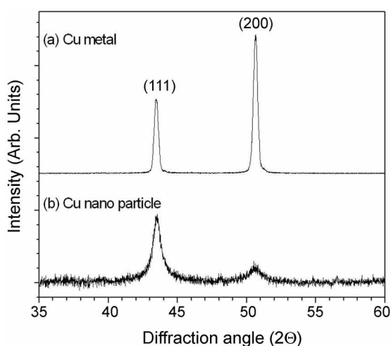
Figure 2. X-ray diffraction profiles of dried suspensions obtained by laser ablation of Cu powder dispersed in 2-propanol.
