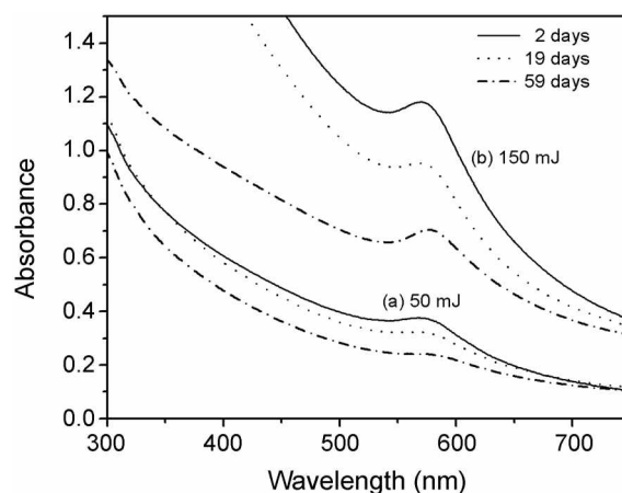
Figure 4. The absorption spectra of Cu nanoparticle solution produced by the second stage irradiation; after 2 days (solid lines), 19 days (dotted lines), and 59 days (dash-dotted lines). The conditions of initial irradiation are 50 mJ/pulse (part a) and 150 mJ/pulse (part b) for 30 min, and that of the second irradiation is 250 mJ/pulse for 50 min.
