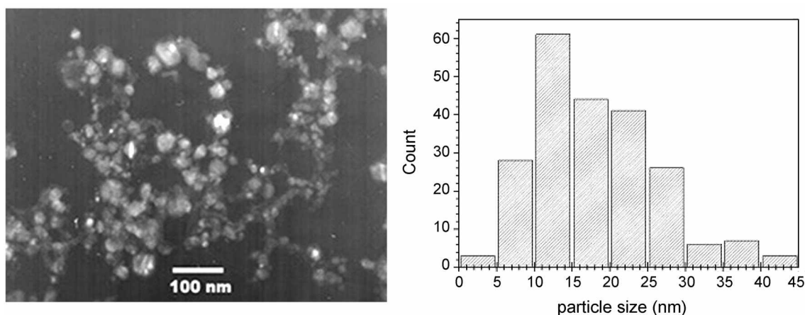
Figure 1. Electron micrographs and size distributions of the Cu nanoparticles produced by laser ablation (532 nm, 100 mJ/pulse, 30 min) of Cu powder dispersed in 2-propanol.
