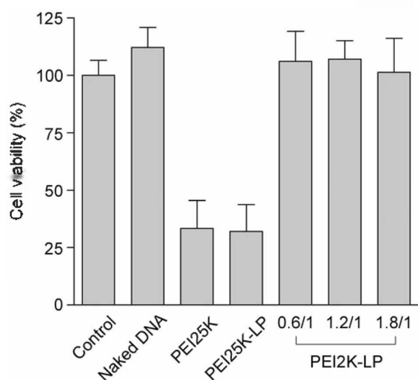
Figure 4. Cytotoxicity of PEI25K, PEI25K-LP and PEI2K-LP. 293 cells were seeded in 96-well microassay plates. PEI25K/DNA (0.8/1), PEI25K-LP/DNA (0.8/1) and PEI2K-LP/DNA complexes were prepared as described in experimental sections. Naked DNA or polymer/DNA complexes were added to the cells and incubated for 4 hrs at 37°C. After the incubation, the transfection mixture was replaced with 100 ml of fresh DMEM medium supplemented with 10% FBS. The cells were incubated for an additional 20 hrs at 37°C. After the incubation, cell viability was measured by MTT assay. The data is expressed as mean values ( \pm standard deviation) of five experiments.
