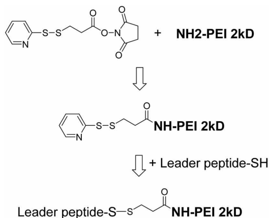
Figure 1. Synthesis scheme of PEI2K-LP.
