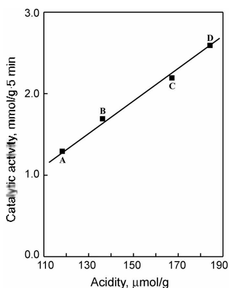
Figure 10. Correlation between catalytic activity for ethylene dimerization and acidity: (A), 5-NiSO 4 /1-CeO 2 -ZrO 2 ; (B), 20-NiSO 4 /1-CeO 2 -ZrO 2 ; (C), 15-NiSO 4 /1-CeO 2 -ZrO 2 ; (D), 10-NiSO 4 /1-CeO 2 -ZrO 2 .
