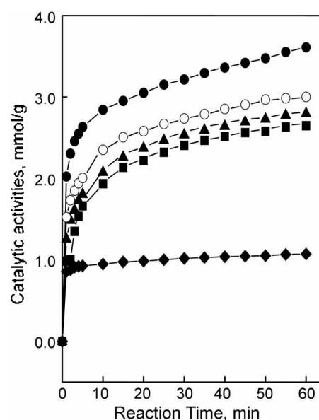
Figure 7. Catalytic activities of 10-NiSO 4 /1-CeO 2 -ZrO 2 as a function of calcination temperature: (●), 600 °C; (○), 700 °C; (▲), 500 °C; (■), 400 °C; (◆), 800 °C.
