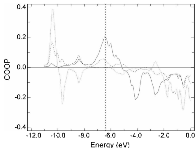
Figure 5. COOP curves for NiTi sublattice after H absorption. Interactions in the upper part are bonding (+), in the lower part antibonding (-). Solid line is Ti-Ti interaction, dotted line Ni-Ni interaction, and dashed line Ni-Ti interaction.
