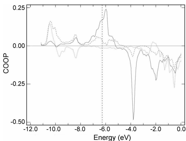
Figure 3. COOP curves for the CsCl-type structure of NiTi. Interactions in the upper part are bonding (+), in the lower part antibonding (-). Solid line is Ti-Ti interaction, dotted line Ni-Ni interaction, and dashed line Ni-Ti interaction.
