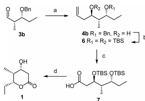
Scheme 1. (a) Allyltributyltin, MgBr 2 ·OEt 2 , CH 2 Cl 2 , RT (91%) (b) (i) Li, di- tert -butylbiphenyl, THF, -78 °C (ii) TBSOTf, 2,6-lutidine (54% in two steps) (c) (i) O 3 , Me 2 S (77%) (ii) NaH 2 PO 4 , NaClO 2 , 2-methyl-2-butene, t -BuOH : H 2 O : THF = 5 : 2 : 10 (98%) (d) 1 M HCl : THF = 5 : 1, 40 °C (70%)
