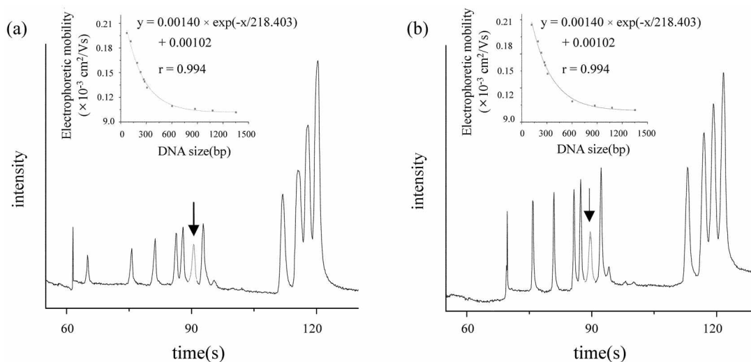
Figure 6. Electropherograms and nonlinear curve fitting for the calculation of the CAG repeat number for (a) a control and (b) an infertile patient. Both 3 \mu\text{L} of 50 ng/mL \Phi\text{X} 174 RF DNA/Hae III and 3 \mu\text{L} of PCR products were placed in reservoir 2. Other conditions were the same as in Figure 2(b).
