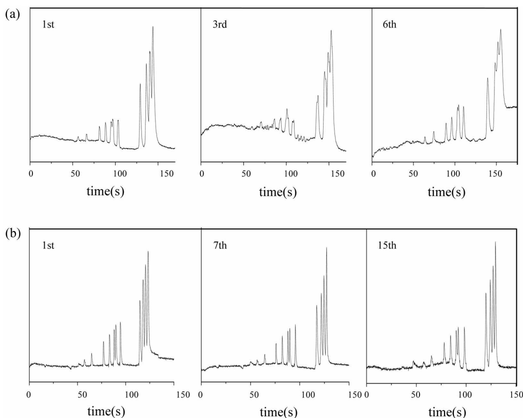
Figure 4. Consecutive running of \Phi X 174 RF DNA/Hae III fragments (a) 1.0% MC, (b) 1.2% PEO. Other conditions were the same as in Figure 2(b).
