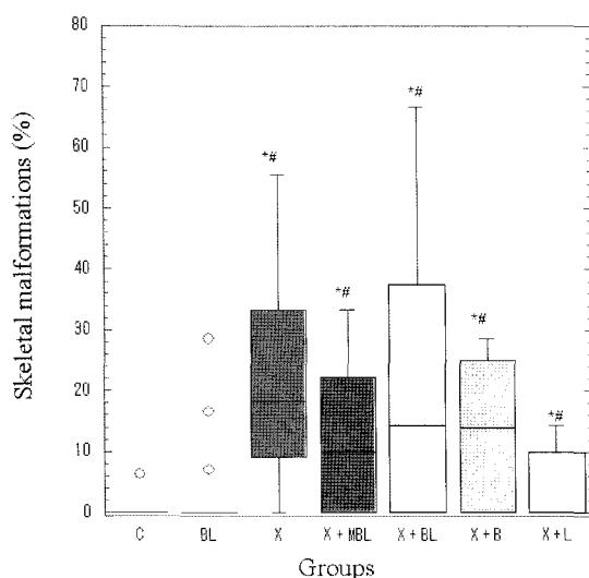
Fig. 3. Skeletal malformations in incidence of ICR mice irradiated at organogenesis period. Each treatment groups were detected with statistical significance ( P < 0.05 ) among all dose groups by Wilcoxon test. C: control (fixation only), LB: EA treatment on the leg and strong transcutaneous stimulation on the back, X: X-irradiation. The X + MBL and X + LB groups were both X-irradiation with EA on the leg and transcutaneous stimulation on the back groups, however they were distinguished according to stimulation intensity on the back. X + MBL group was treated with mild stimulator that gave mild twitching. X + LB group was treated with strong stimulation that gave severe twitching. X + B: X-irradiation with strong transcutaneous stimulation on the back, X + L: X-irradiation with EA on the leg.
