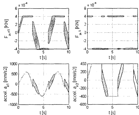
Fig. 4 Friction force from friction element used in Vampire
