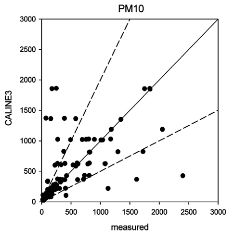
Fig. 6. Comparison of measured PM10 concentrations with the predicted ones by CALINE3 in flat terrain.
