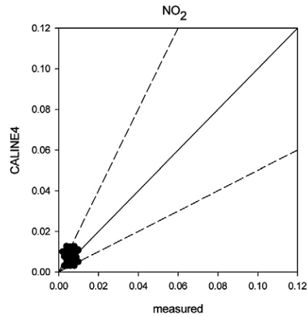
Fig. 11. Comparison of measured NO 2 concentrations with the predicted ones by CALINE4 in bridge terrain.
