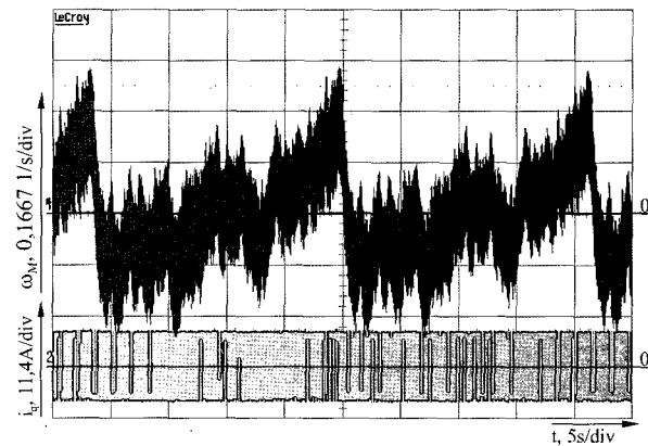
Fig. 10 Measured speed and excitation PRBS
