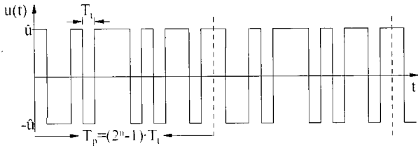
Fig. 3 PRBS signal u(t)
