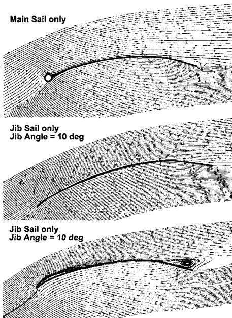
Fig. 9 Streamlines over jib and main sails (on the section of 25% Height)
