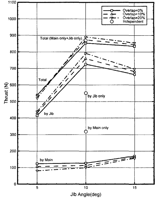
Fig. 19 Thrust by sail sets
