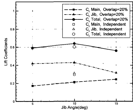
Fig. 12 Lift changed by jib angle
