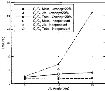
Fig. 14 L/D changed by jib angle
