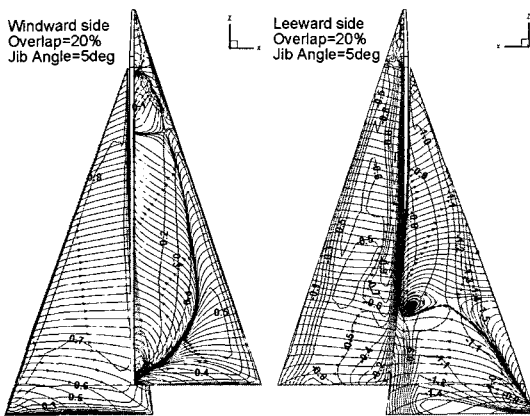
Fig. 10 Cp Contours and limiting streamlines changed by jib angle (Overlap=20%)
