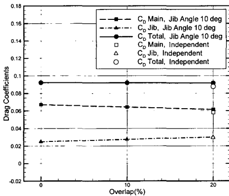
Fig. 18 Drag changed by overlap
