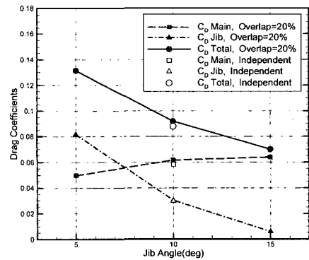
Fig. 13 Drag changed by jib angle
