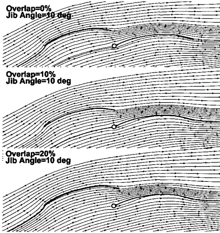
Fig. 16 Streamlines changed by overlap (Jib angle=10 deg)
