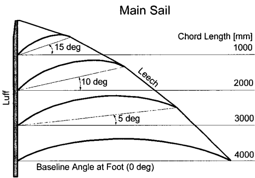
Fig. 2 Geometry of main sail
