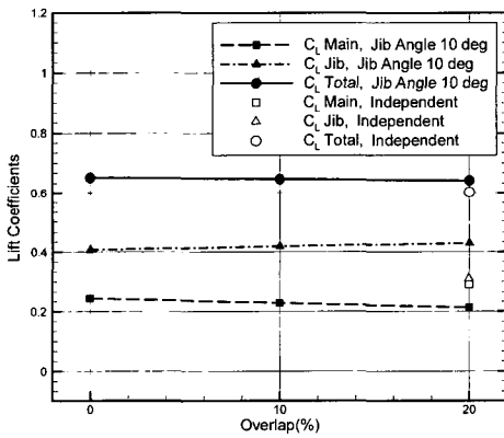
Fig. 17 Lift changed by overlap
