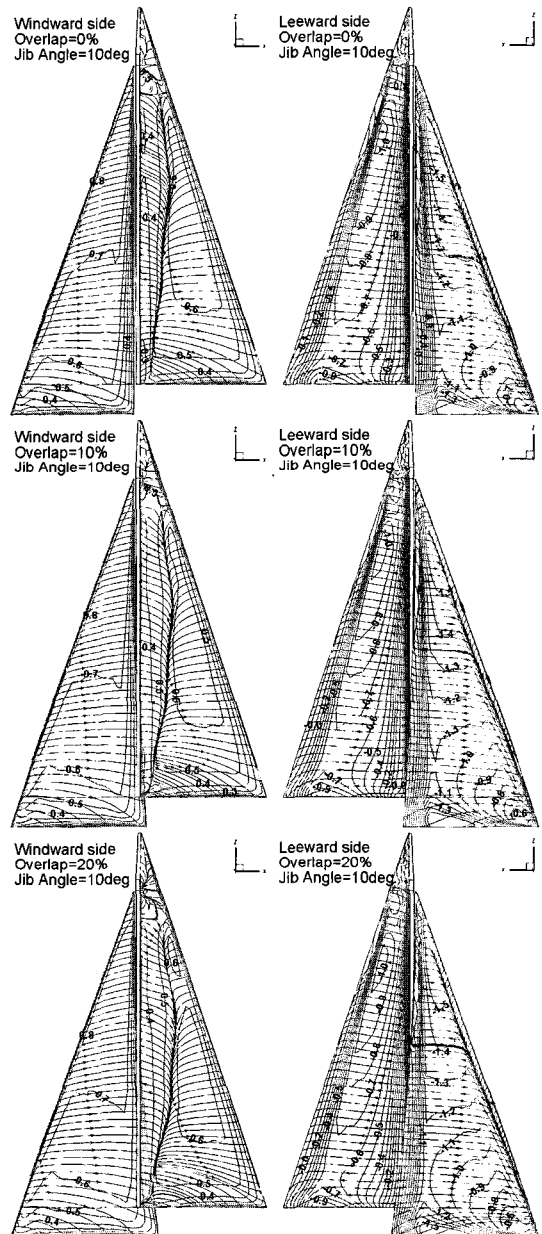
Fig. 15 Cp Contours and limiting streamlines changed by overlap (Jib angle=10 deg)
