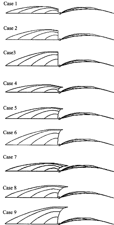
Fig. 5 Geometries of sail sets(Top view)
