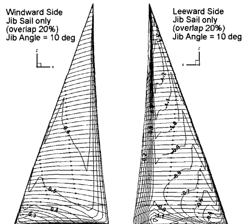
Fig. 7 Cp Contours and limiting streamlines on jib sail only(Case 8, Jib Angle=10 deg)
