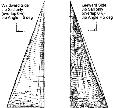
Fig. 8 Cp Contours and limiting streamlines on jib sail only(Case 1, Jib Angle=5 deg)
