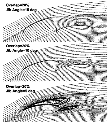
Fig. 11 Streamlines changed by jib angle (20% overlap)
