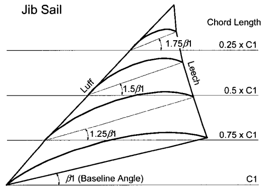
Fig. 3 Geometry of jib sail
