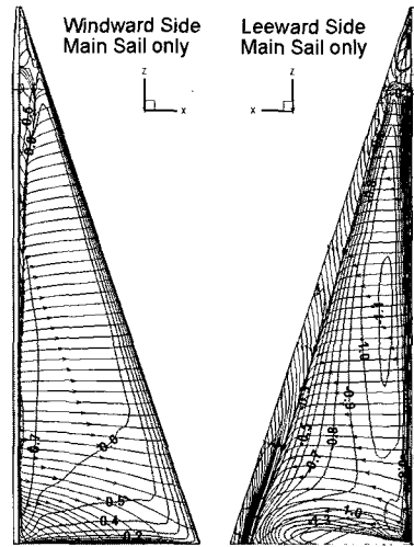
Fig. 6 Cp Contours and limiting streamlines on main sail only
