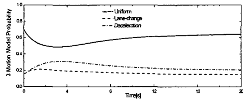
(b) Probability of three motion models
