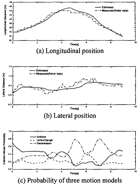
Fig. 4 Target state estimation of a rapidly braking vehicle
