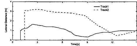
(b) Lateral position (Probability-based method)
