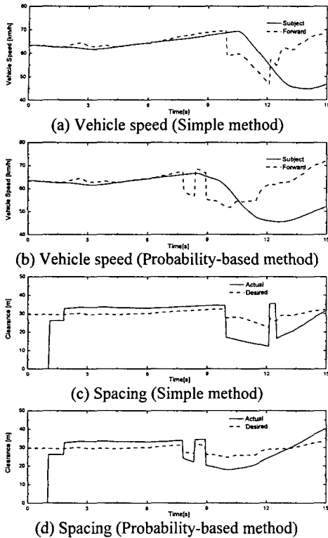
Fig. 8 Control results : simple method versus probability-based method
