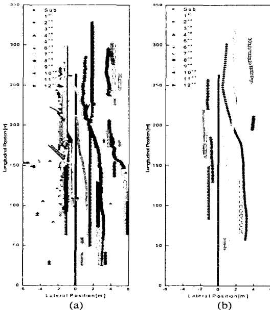
Fig. 6 MTT-ACC simulation results using driving data of a cut-in situation. (a) Data tracks from mmW radar (b) Estimated IMM-PDAF tracks
