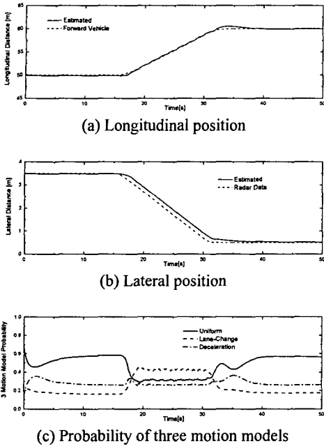
Fig. 3 Target state estimation of a vehicle performing a lane change
