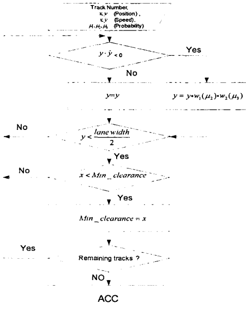
Fig. 5 Flowchart of the primary target determination algorithm
