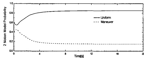
(c) Probability of two motion models
