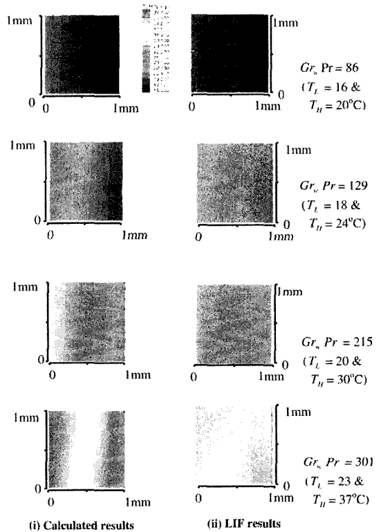
Fig. 8 Temperature field for the top region of a heated channel
