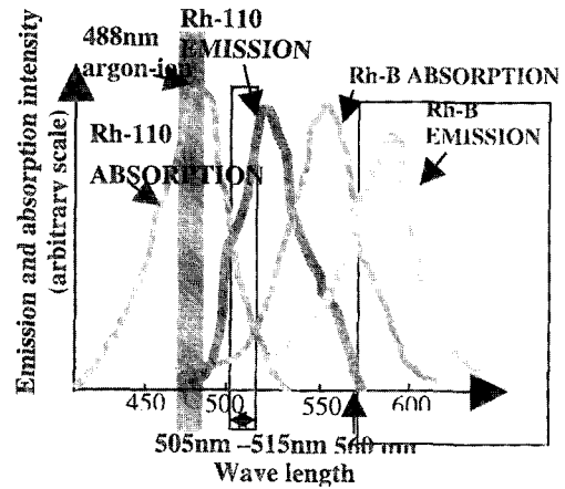
Fig. 1 Absorption and fluorescence spectra of Rhodamine-110 and Rhodamine-B
