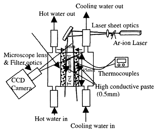
Fig. 5 Experimental Apparatus for MPIV and 2-color LIF
