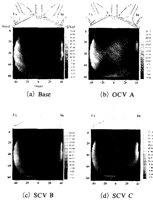
Fig. 12 Mean kinetic energy distribution in cylinder (L=8 mm)
