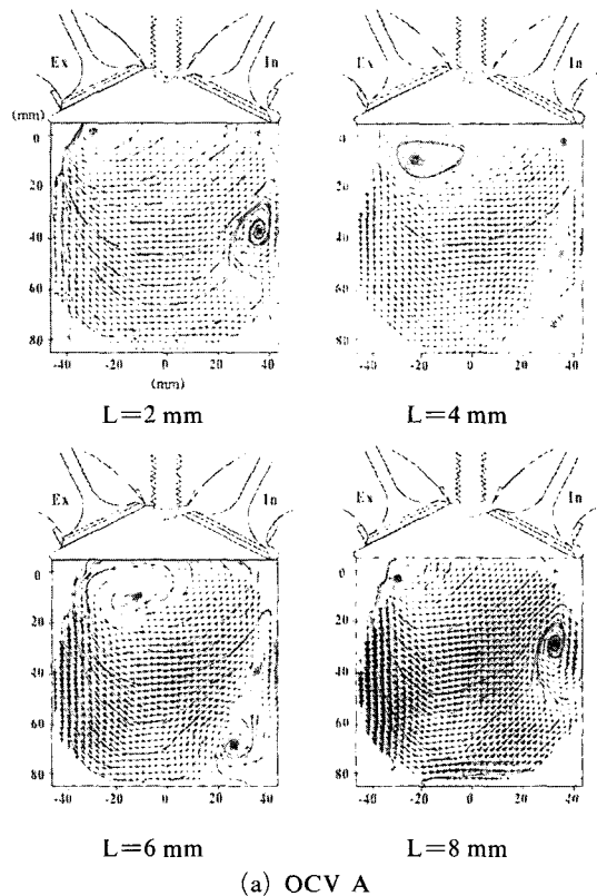
Fig. 11 Ensemble averaged velocity field and streamlines (a) OCV A
