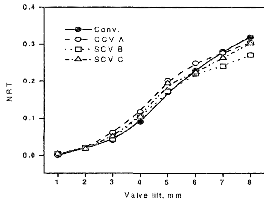
Fig. 7 Effects of OCV and SCV configuration on non dimensional rig tumble
