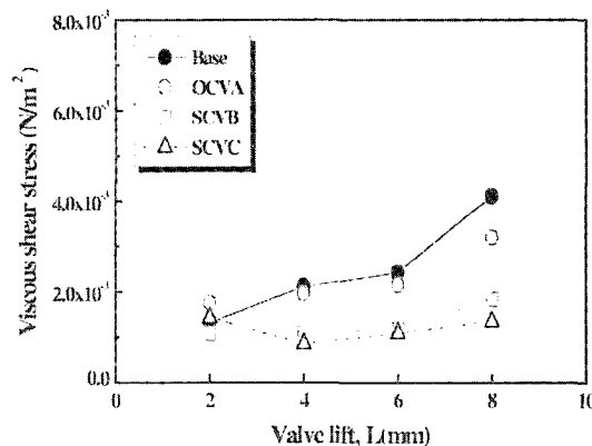
Fig. 18 Comparison of viscous shear stress according to valve lift
