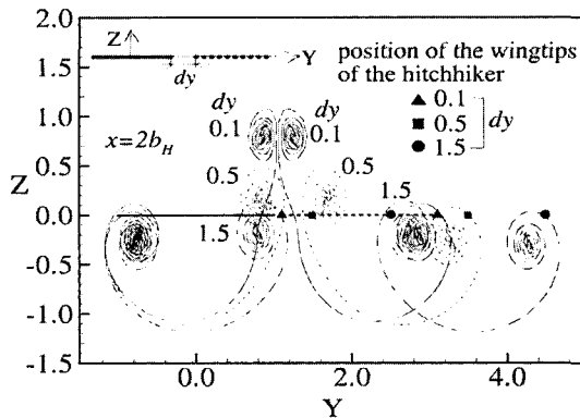
Fig. 5 Effect of gap on the positions of the wingtip vortices behind elliptically loaded wings in close formation flight, when two wings have the same wing loadings ( \Gamma_0^M = \Gamma_0^H = 1.0 , b_M = 1.0 , dz=0.0 , dt=0.01 , N=400 , OGE)
