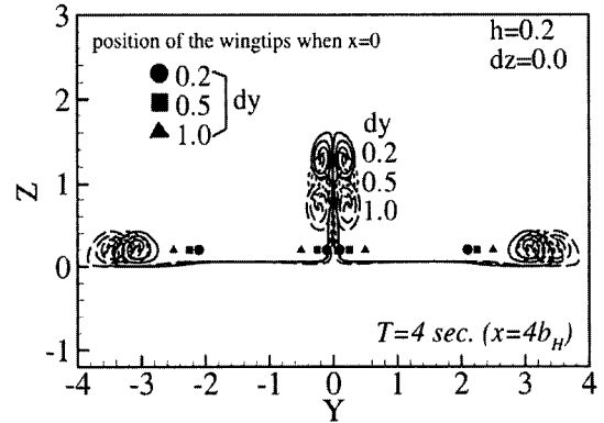
Fig. 6 Effect of gap on the positions of the wingtip vortices behind elliptic wings in close formation flight ( \Gamma_0^M = \Gamma_0^H = 1 and b_M = b_H = 2.0 , dz=0.0 , dt=0.01 , N=400 , IGE)
