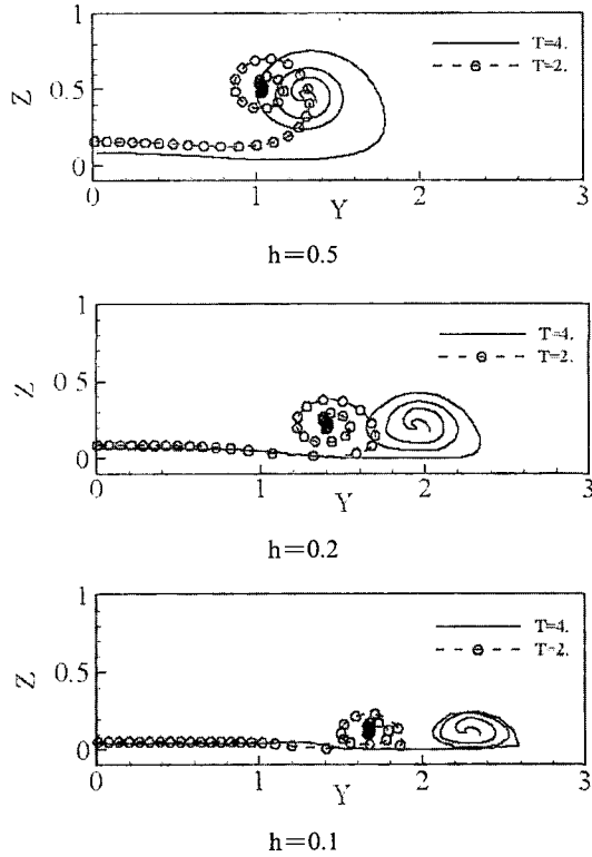
Fig. 4 Ground effect on the unsteady evolution of the vortex sheets ( N=200 , \delta t=0.01 )
