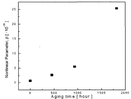
Fig. 10 Effect of aging time on non-linear parameter ( \beta )
