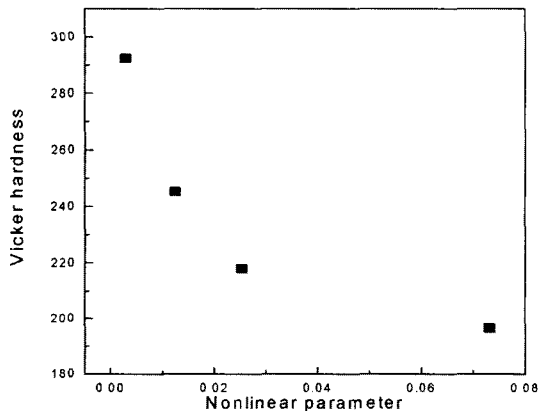
Fig. 18 Relation between non-linear parameter and Vickers hardness
