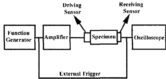
Fig. 9 Block diagram of apparatus for non-linear ultrasonic test
