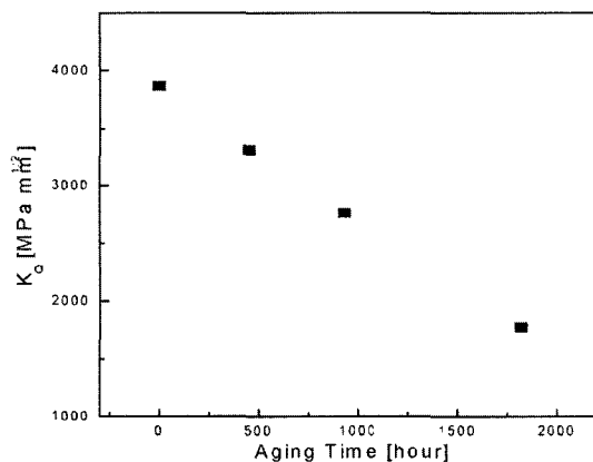
Fig. 4 Effect of aging time on fracture toughness
