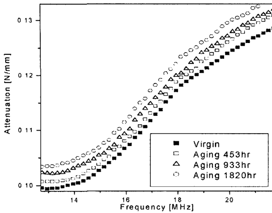
Fig. 7 Effect of frequency on attenuation coefficient
