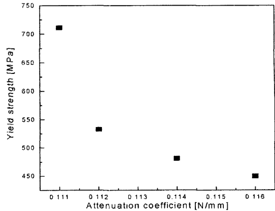
Fig. 11 Relation between yield strength and attenuation coefficient
