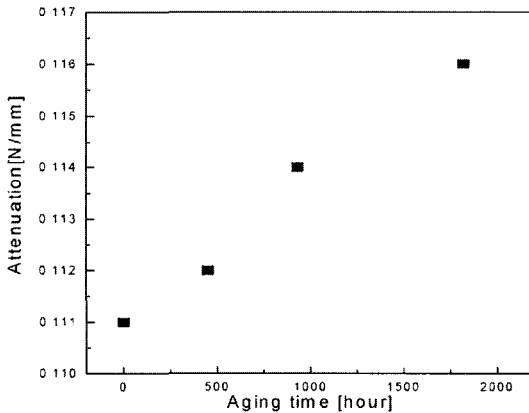
Fig. 8 Effect of aging time on attenuation coefficient at center frequency
