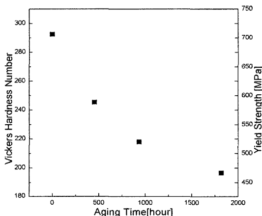
Fig. 5 Effect of aging time on Vickers hardness and yield strength.
