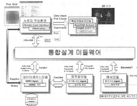
Fig 3. System Architecture
