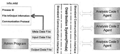
Fig 4. Integrated Analysis Code
