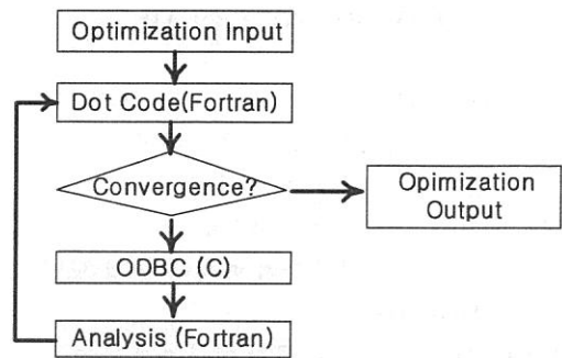
Fig8 . Integrated Optimization Code
