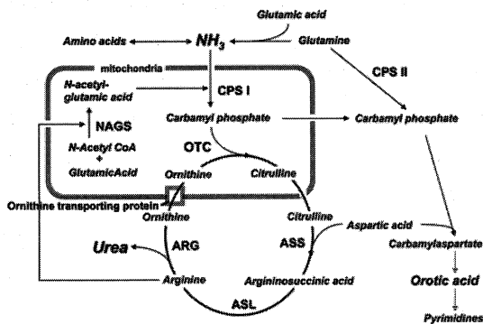
Fig. 1. The urea cycle. ASL, argininosuccinate lyase; ARG, arginase; NAGS, N-acetylglutamate synthetase.
