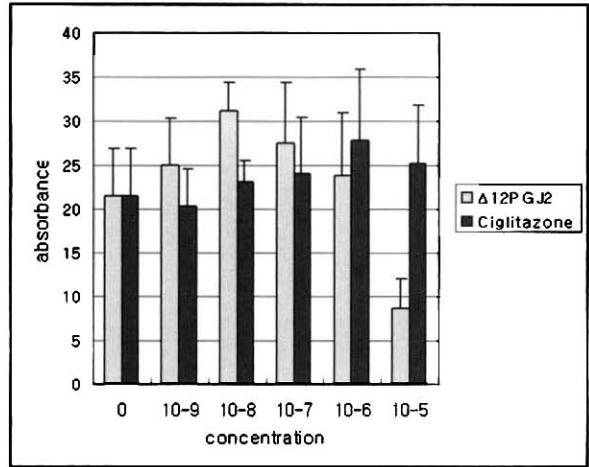
Figure 2. Effect of the concentration of \Delta^{12}\text{PGJ}_2 and ciglitazone on the proliferation of Saos-2 cells at day 2
