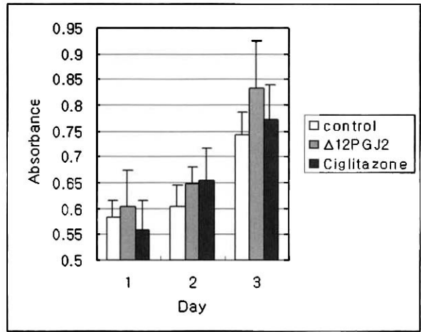
Figure 3. Effect of the \Delta^{12}\text{PGJ}_2 and ciglitazone on time-course proliferation
