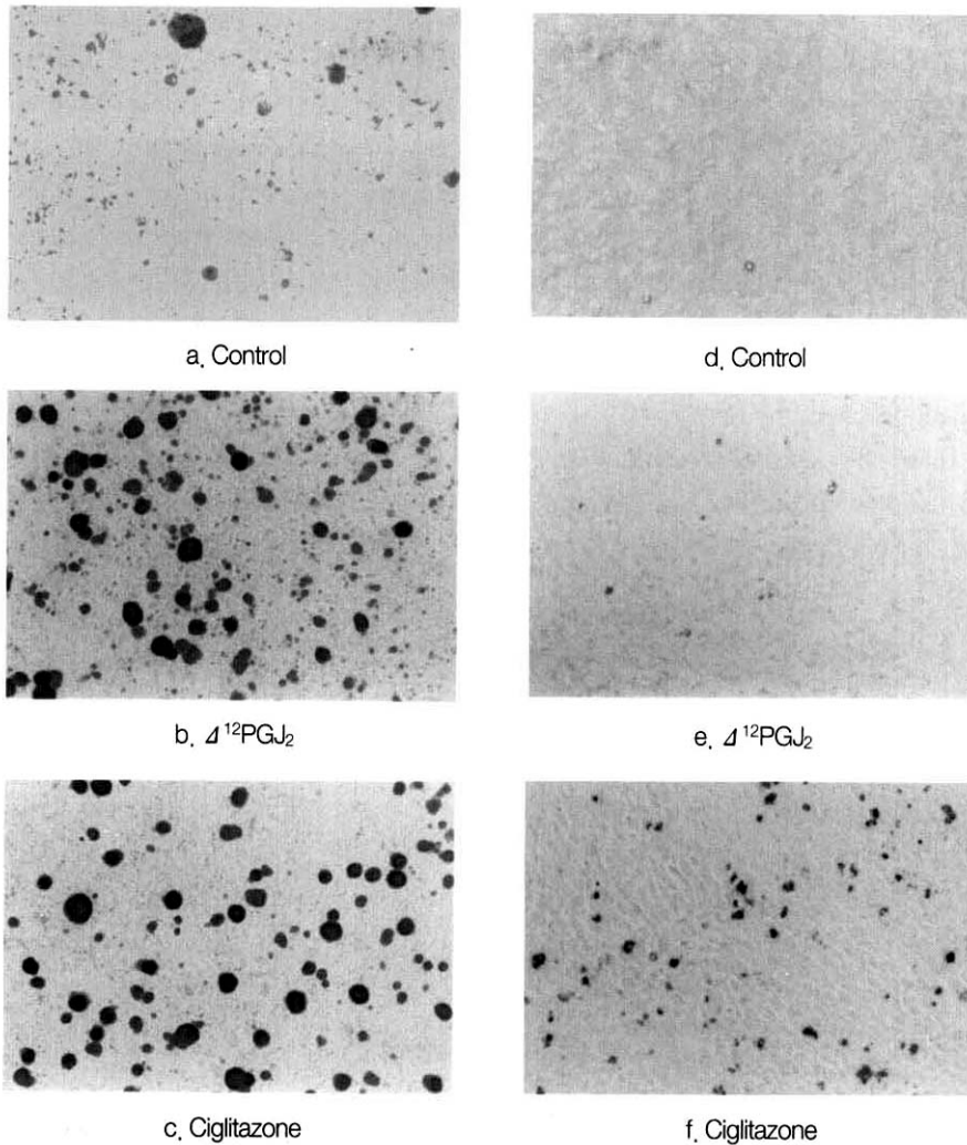
Figure 7. Effects on mineralization of MC3T3-E1 cells (X100, a, b, c - Alizarin red S stain / d, e, f- von Kossa stain)
