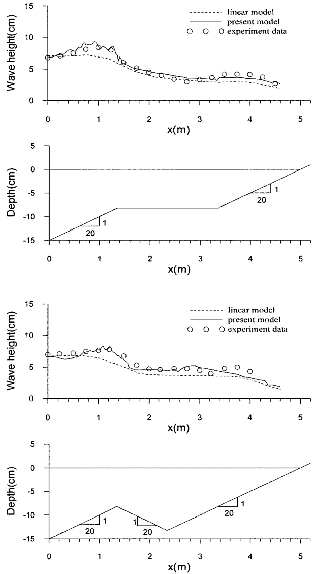
Fig. 2 Wave deformation across the surf zone according to change of slope
