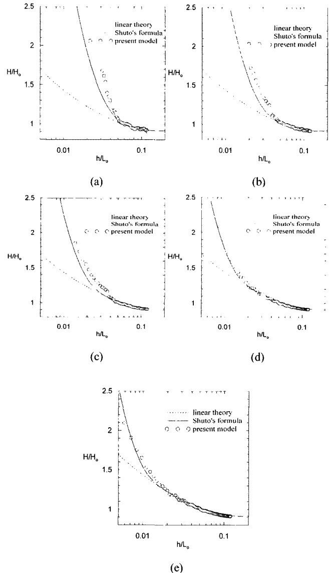
Fig. 1 Shallowing coefficient for (a) H_0/L_0=0.02 , (b) H_0/L_0=0.01 , (c) H_0/L_0=0.005 , (d) H_0/L_0=0.002 , (e) H_0/L_0=0.001
