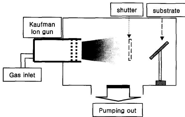
Fig. 1. The ion beam (Kaufman type) exposure system.
