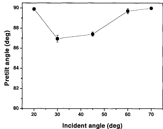
Fig. 3. Generation of pretilt angles in NLC with IB exposure on the SiC thin film surfaces for 1 min as a function of incident angle.
