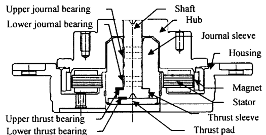
Fig. 1 Rotating-shaft type of a HDB spindle motor
