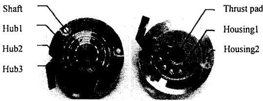
Fig. 6 Temperature measurement around the periphery of the HDB spindle motor
