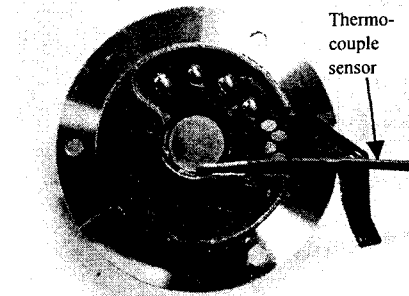
Fig. 8 HDB spindle motor with a thermocouple sensor
