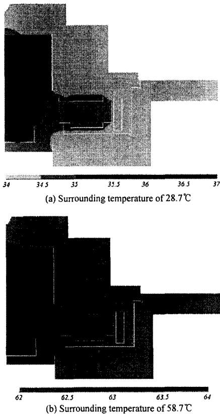
Fig. 9 Temperature distribution of the HDD spindle motor
