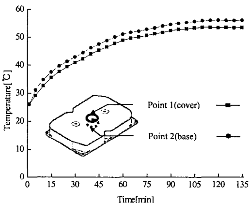
Fig. 2 Temperature variation on the top-cover and base of a HDD inside a computer
