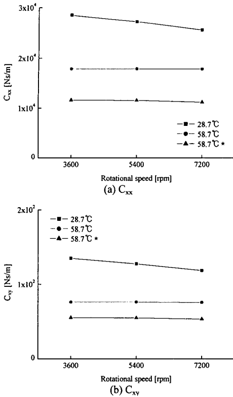
Fig. 12 Variation of the damping coefficients of the upper journal bearing (* means the damping coefficients without considering the clearance variation)
