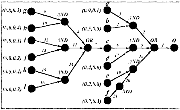
Figure 17. Sequential Search of Inference Network
