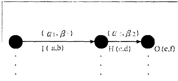
Figure 8. Construction of fuzzy Inference Network
