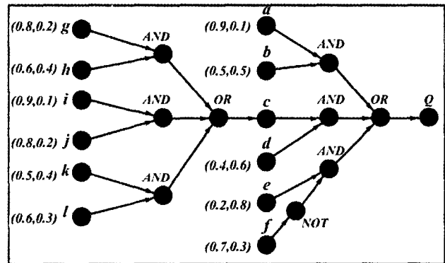
Figure 15. Construction of Fuzzy Inference Network
