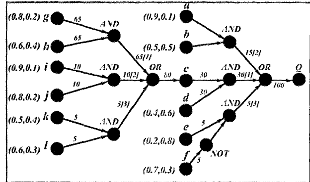
Figure 18. Search by priority in Fuzzy Inference Network
