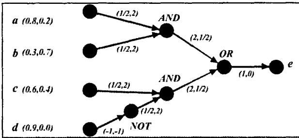
Figure 13 An Example of Fuzzy Inference Network
