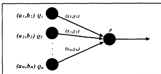
Figure 2. propagation rule for Neural Logic Network
