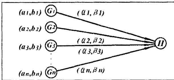
Figure 14. Propagation of Node Values in Fuzzy Inference Network
