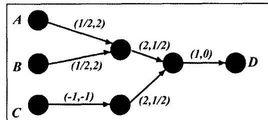
Figure 7. Representation of a rule using Neural Logic Network
