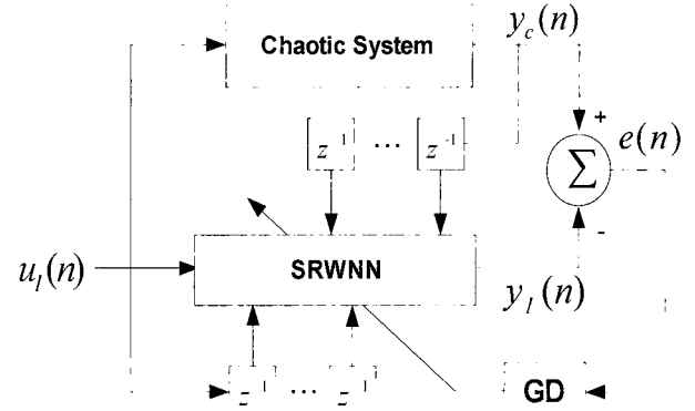
Fig. 2. Identification structure using the SRWNN.
