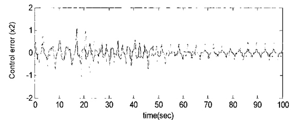
Fig. 5. The control errors of the SRWNN(solid line) and WNN(dotted line).
