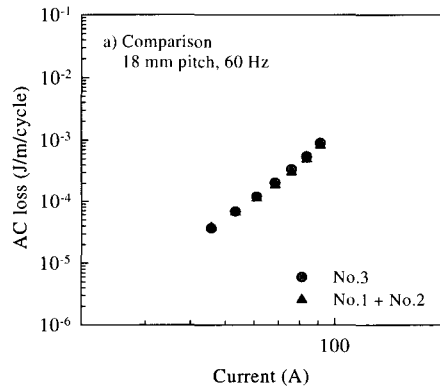
Fig. 3. Voltage lead's arrangement dependence of the AC losses in the helical coil with a 18 mm pitch.
