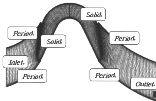
Fig. 1. Geometry & grid system with a far-field inlet boundary condition
