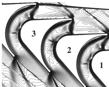
(c) Mach contours for a linear nozzle
