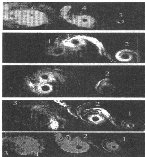
Fig. 1. Sequence of tip-vortex pairing from the individual blade, 9^\circ collective, 3.5 fps climb rate (Ref. 6)
