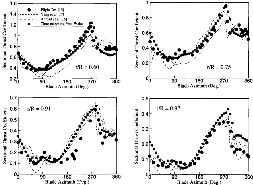
Fig. 7. Sectional thrust coefficient comparisons for AH-1G rotor
