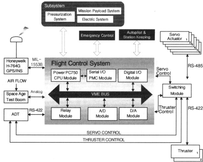
Fig. 2. AFCS Structure
