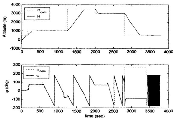
Fig. 21. Simulation Results for Altitude and Heading Angle
