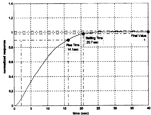
Fig. 14. Normalized Step Response of Airspeed Hold Mode
