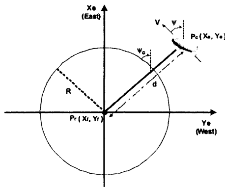
Fig. 18. Guidance Logic for Turning Flight
