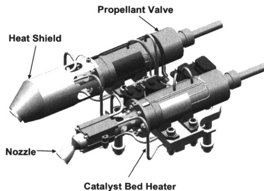
Fig. 3. Configuration of Dual Thruster Module
