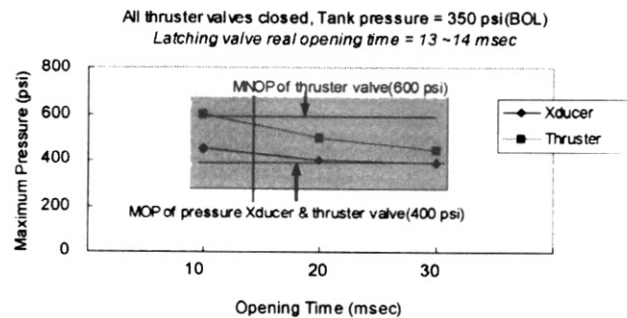
Fig. 7. Max. Pressure Estimations of Propellant Flow
