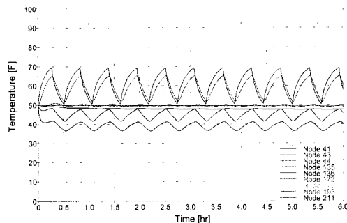
Fig. 6. Thermal Behavior of Propellant Tank
