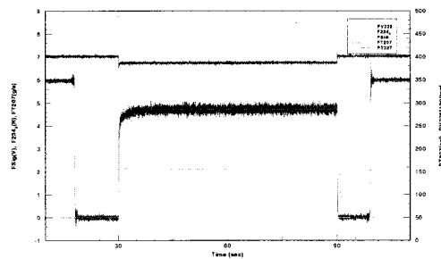
(b) Measured Results of Thruster Performance
