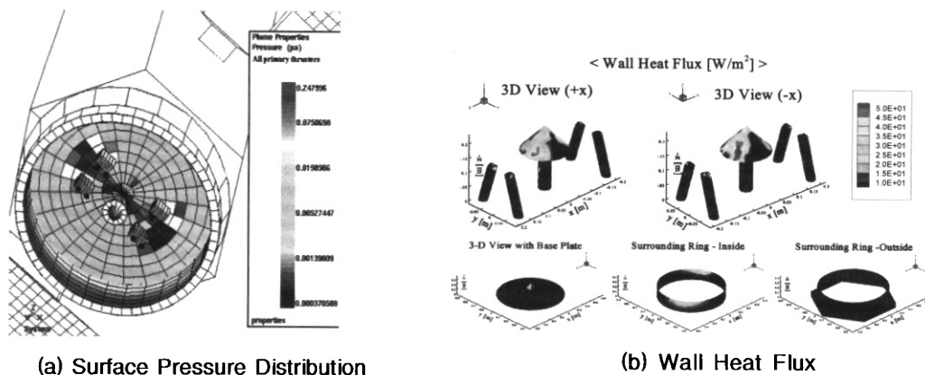
Fig. 8. Thruster Exhausted Plume Analysis Results
