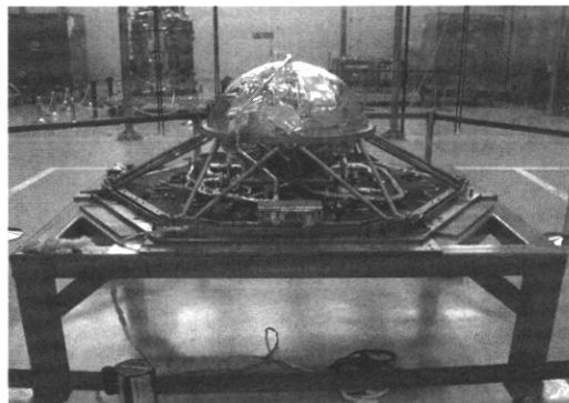
Fig. 12. Final Configuration of PS Assembly
