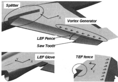
Fig. 8. Proposed Aerodynamic Devices
