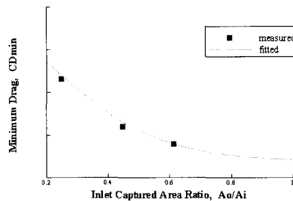
Fig. 7. Spillage Drag Distributions
