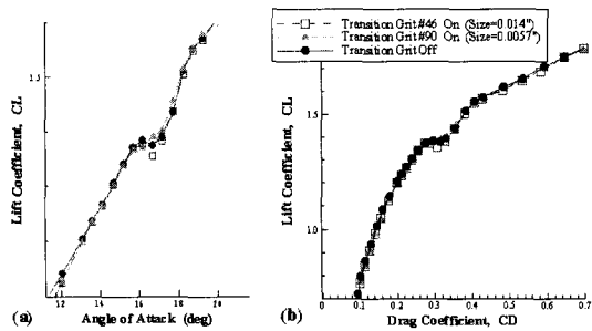
Fig. 27. Effect of Transition Grits (LEF/TEF=30°/20°)
