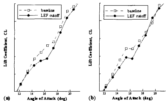
Fig. 21. Effect of Leading Edge Flap Cutoff (LEF/TEF= 30^{\circ}/20^{\circ} , Sideslip= 10^{\circ} )
