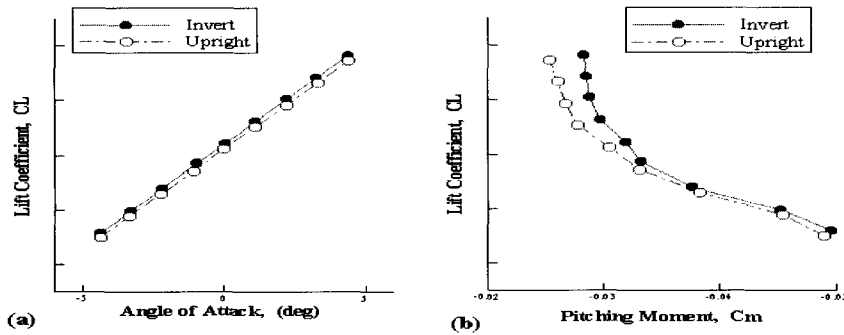
Fig. 5. Flow Angularity Effect on Lift and Pitching Moment
