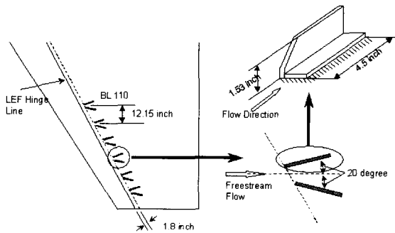
Fig. 11. Vortex Generators on Wing
