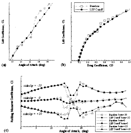
Fig. 20. Effect of Leading Edge Flap Cutoff (LEF/TEF= 30^{\circ}/20^{\circ} )
