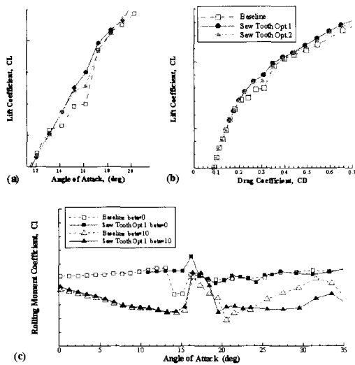
Fig. 22. Effect of Saw Teeth (LEF/TEF=30°/20°)
