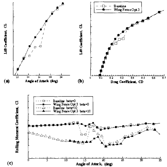
Fig. 25. Effect of Boundary Layer Fence Option.3 (LEF/TEF=30°/20°)
