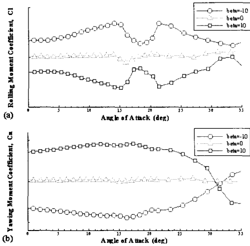
Fig 16. Lateral and Directional Characteristics at Up-and-Away Condition (LEF/TEF=30°/0°)
