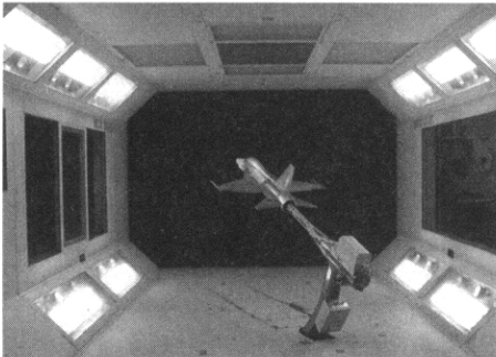
Fig. 3. T-50 Model in W/T Test Section
