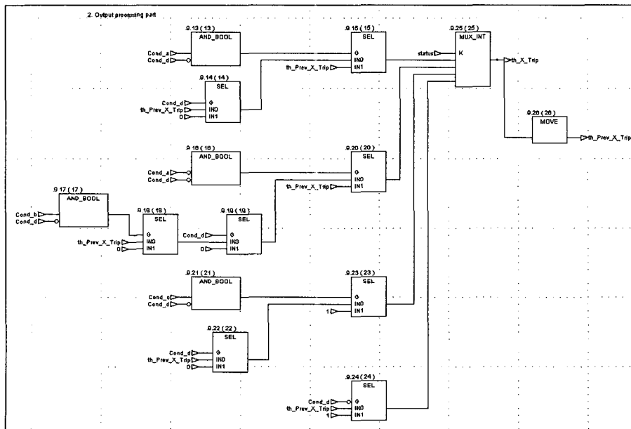
(b) Output processing part FBD
