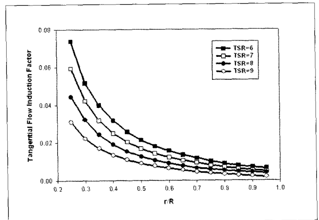
Fig. 6 Tangential flow induction factors (using measured lift & drag coefficient)
