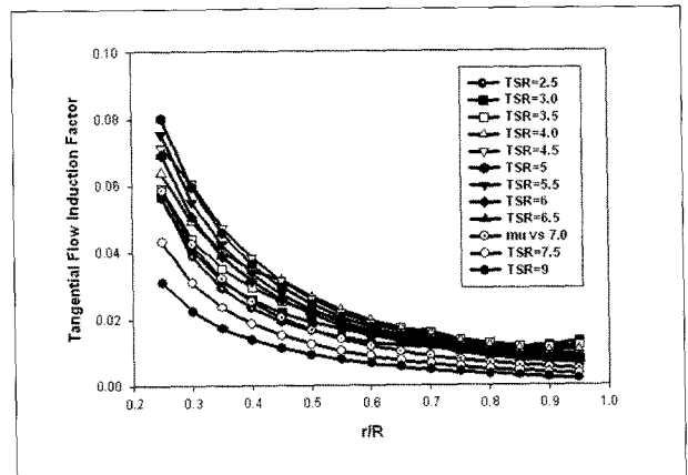
Fig. 7 Tangential flow induction factors (using predicted lift & drag coefficient)
