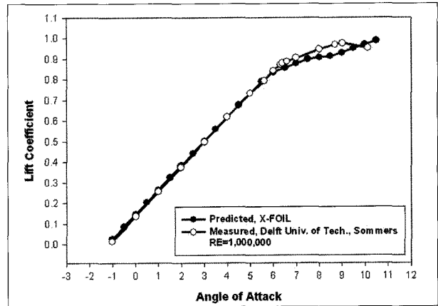
Fig. 2 Lift coefficient comparison (S809)
