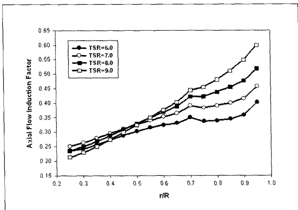
Fig. 4 Axial flow induction factors (using measured lift & drag coefficient)
