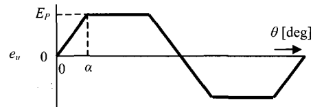
Fig. 2 Trapezoidal electro-motive force
