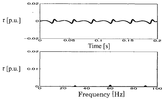
Fig. 11 Simulation results of the proposed voltage ( \gamma=0.19 )
