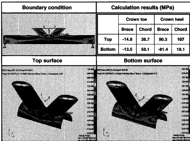
Fig. 4 Nominal stress distribution under 392kN concentrated load
