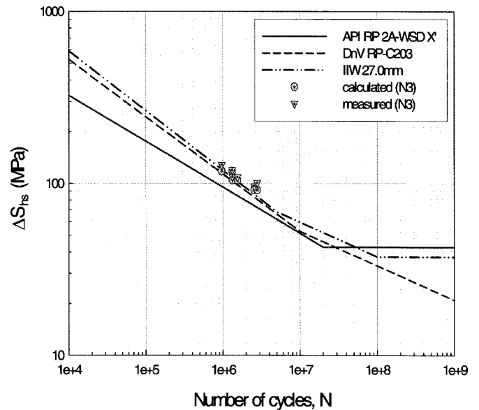
Fig. 9 \Delta S_{hs} -N 3 curve
