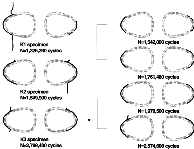
Fig. 6 Fatigue crack propagation
