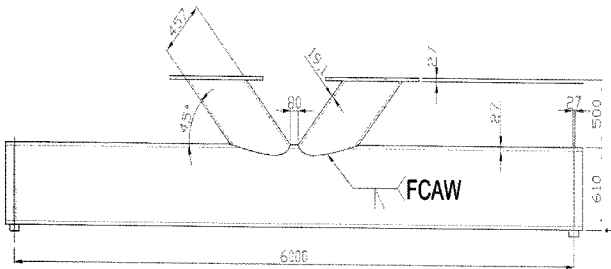
Fig. 1 K joint test specimen
