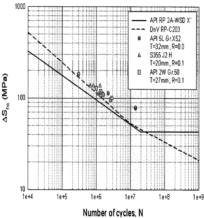
Fig. 10 \Delta S_{hs}-N_3 curve of YS 355MPa steel materials
