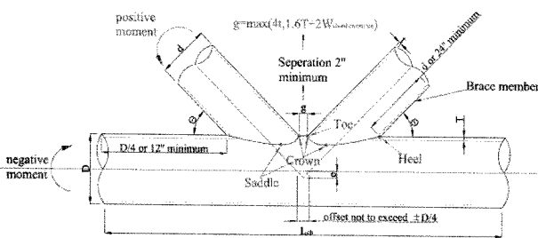
Fig. 2 Detail of Tubular K joint
