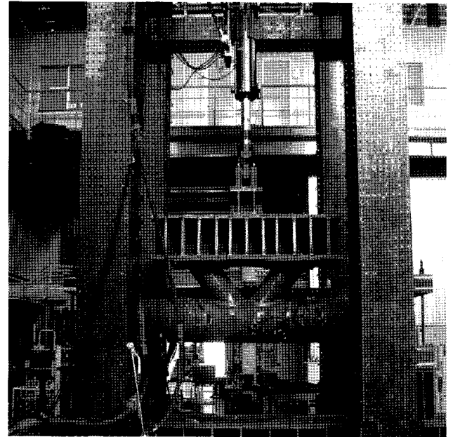
Fig. 3 Test specimen Setting
