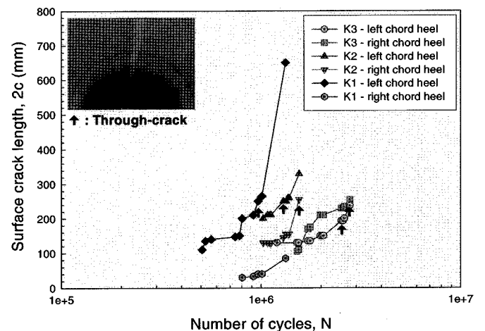
Fig. 8 Crack length vs Number of cycles
