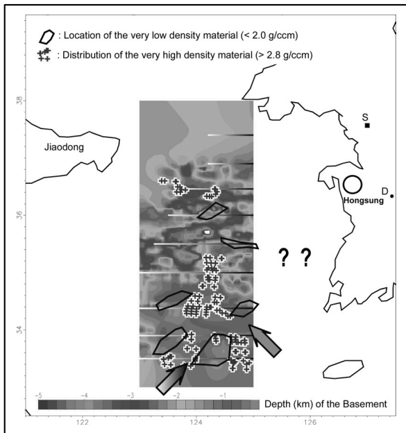
Fig. 2 The depth distribution of the model-Basement and the location of the very high and very low material in the investigations area.
