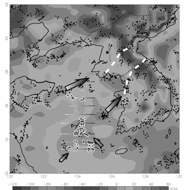
Fig. 3 CHAMP-GRACE Gravity Anomaly in Yellow Sea and Korean peninsula. black points indicate the location of source structures with an average depth of 20 km calculated by Euler method. Here shown the anticipated collision's boundary between North and South China block
