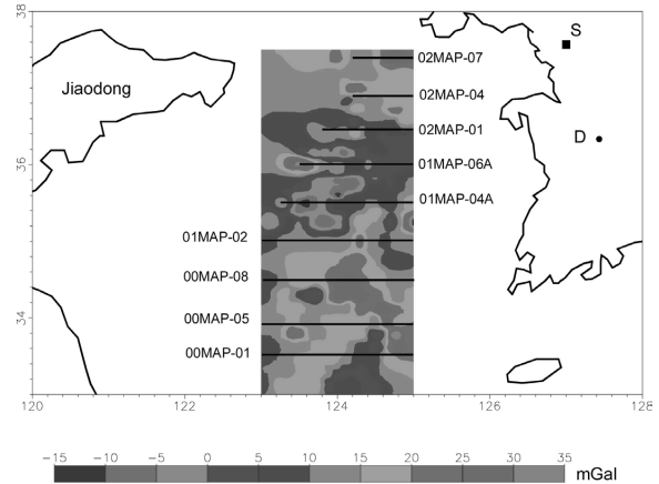
Fig. 1 Free Air anomaly over the Yellow Sea Basin and the location of the seismic cross section (GIGAM, 2002).
