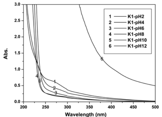
Fig. 5. Variation of UV/VIS spectra depending on pH from wastewater purified with the powdered activated carbons treated with potassium salts (K1).
