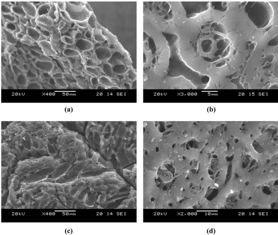
Fig. 2. SEM images obtained from powdered activated carbons treated with potassium salts; (a) K1 ( \times 400 ), (b) K1 ( \times 3000 ), (c) K2 ( \times 400 ) and (d) K2 ( \times 2000 ).
